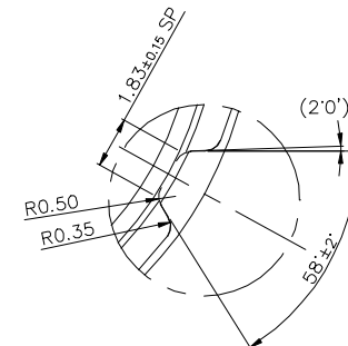
PRESSURE RELIEF GROOVE DETAIL-"B" SCALE - 5:1
