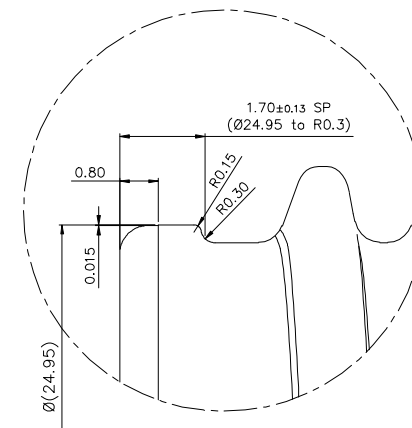
DETAIL-C SCALE - 5:1
