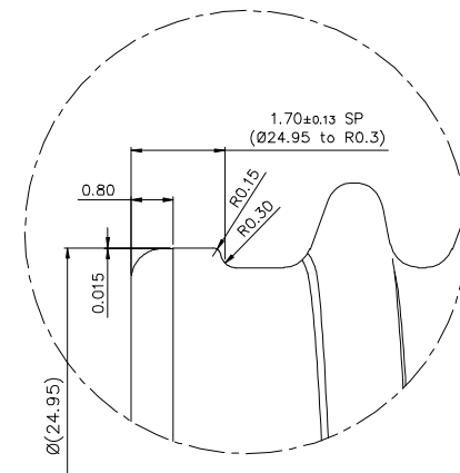
DETAIL-C SCALE - 5:1
