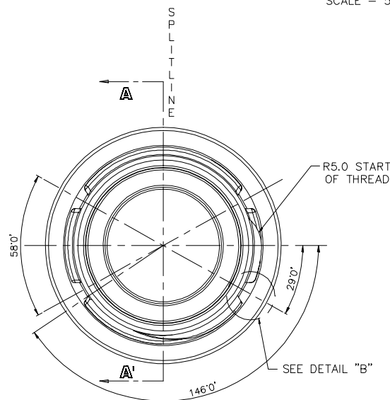
VIEW FROM-X SCALE - 2:1
