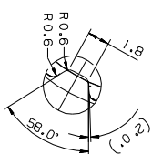
DETAIL B M 5:1 PRESSURE RELIEF GROOVE
